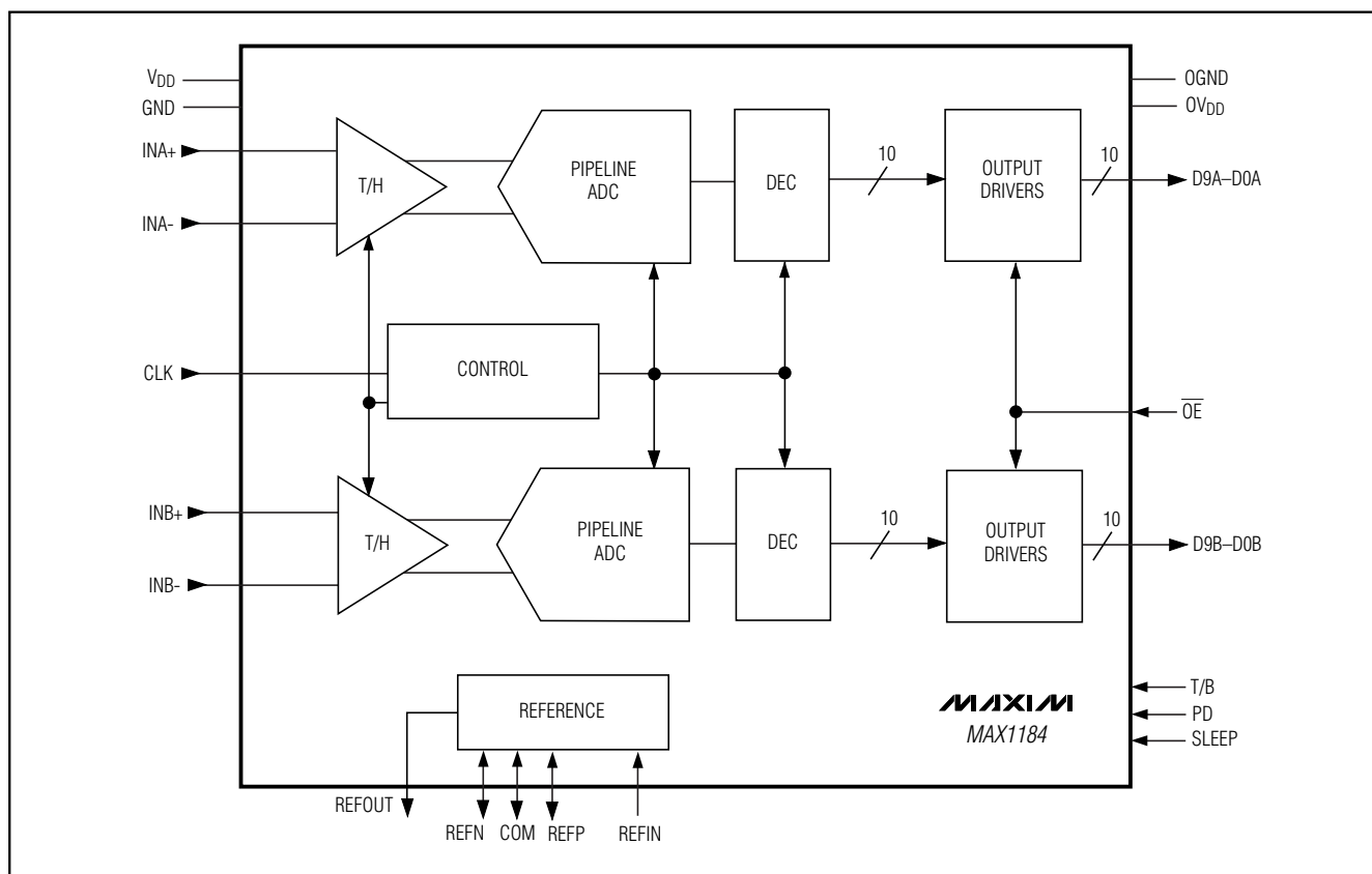
Functional Diagram
