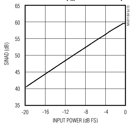
SIGNAL-TO-NOISE + DISTORTION vs. INPUT POWER ( f_{IN} = 7.5343935MHz )
