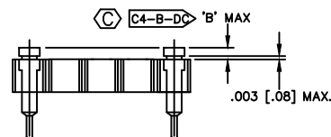
FIGURE 8 OPTION -N (FOR -SD STYLE, SEE NOTE 9 SHT.1) (FOR HSS AND SS STYLES, SEE NOTES 3 & 4) 'B' DIMENSION FOR OPTION -N = NON FLUSH
