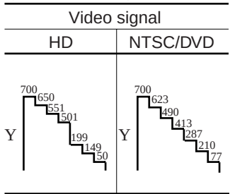
Analog YUV signal (HD/NTSC/DVD)
