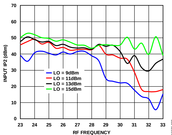
Figure 20. Input IP2 vs. RF Frequency at Various LO Power Levels, T_A = 25^\circ\text{C}
