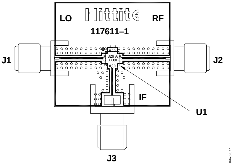
Figure 74. Evaluation PCB Top Layer
