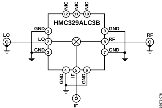
Figure 73. Typical Application Circuit
