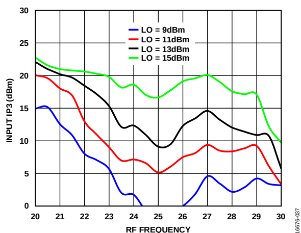
Figure 34. Input IP3 vs. RF Frequency at Various LO Power Levels, T_A = 25^\circ\text{C}
