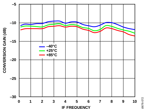
Figure 69. Conversion Gain vs. IF Frequency at Various Temperatures, LO = 13 dBm
