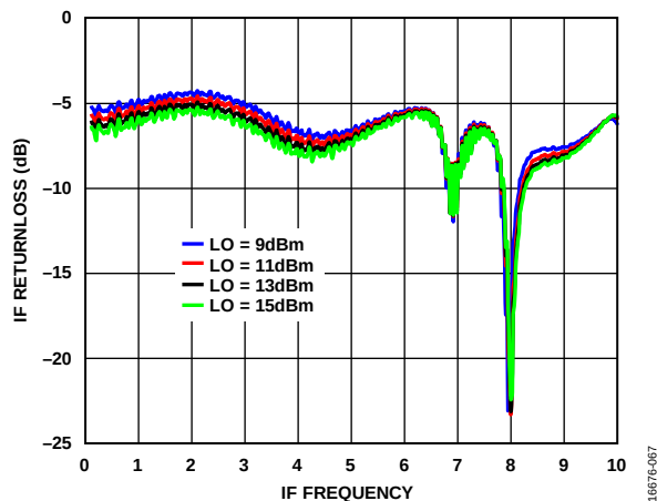
Figure 64. IF Return Loss vs. IF Frequency at Various LO Power Levels, T_A = 25^\circ\text{C} , LO = 27 GHz
