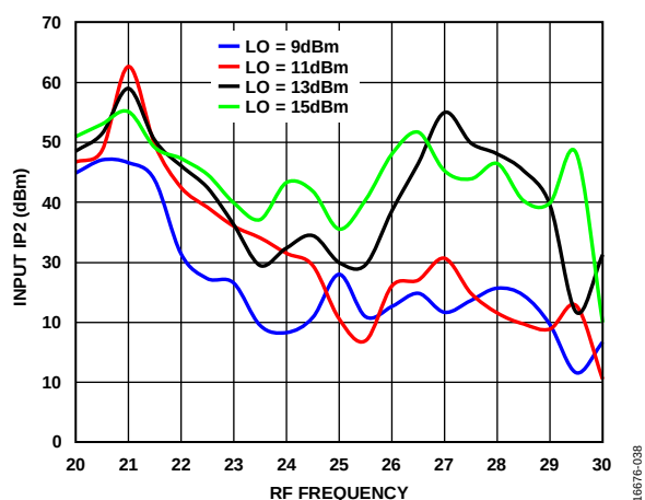
Figure 35. Input IP2 vs. RF Frequency at Various LO Power Levels, T_A = 25^\circ\text{C}
