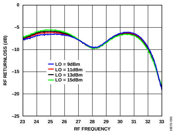
Figure 63. RF Return Loss vs. RF Frequency at Various LO Power Levels, T_A = 25^\circ\text{C} , LO = 27 GHz
