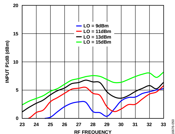
Figure 47. Input P1dB vs. RF Frequency at Various LO Power Levels, T_A = 25^\circ\text{C}
