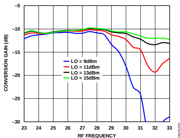
Figure 18. Conversion Gain vs. RF Frequency at Various LO Power Levels, T_A = 25^\circ\text{C}
