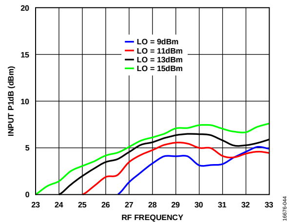
Figure 41. Input P1dB vs. RF Frequency at Various LO Power Levels, T_A = 25^\circ\text{C}
