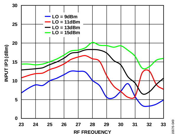
Figure 46. Input IP3 vs. RF Frequency at Various LO Power Levels, T_A = 25^\circ\text{C}
