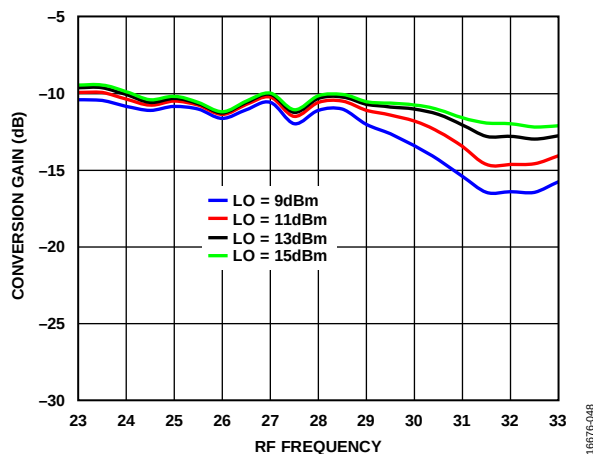
Figure 45. Conversion Gain vs. RF Frequency at Various LO Power Levels, T_A = 25^\circ\text{C}
