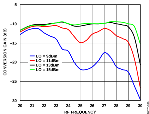
Figure 33. Conversion Gain vs. RF Frequency at Various LO Power Levels, T_A = 25^\circ\text{C}
