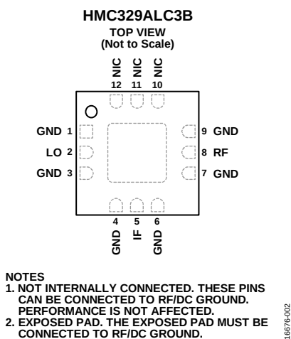
Figure 2. Pin Configuration
