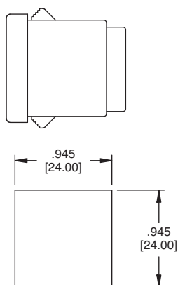
Recommended Panel Cut-Out For Panel 0.8mm - 1.50mm
