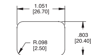
Recommended Panel Thickness: 0.80mm - 3.0mm
