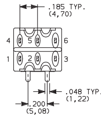
8261SH9ABE2 DPDT
