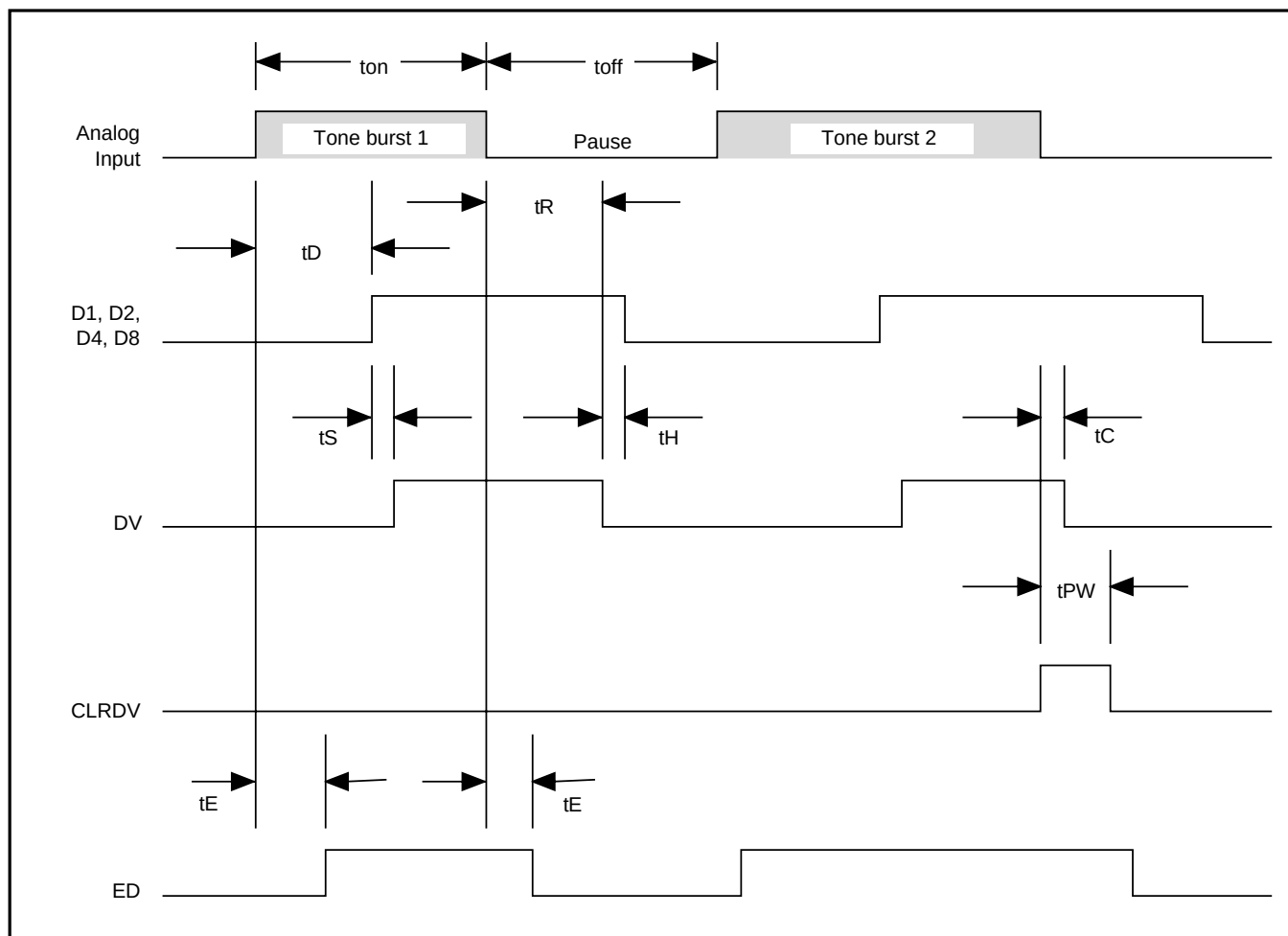
FIGURE 4: Timing Diagram
