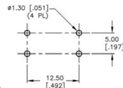
P.C. MOUNTING
