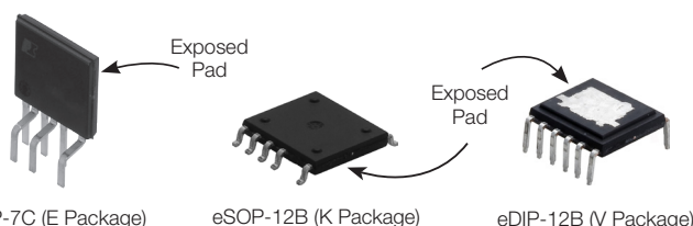
Figure 2. Package Options.
