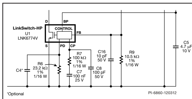
Figure 13. 17 W LCD Monitor Supply (+18 V, +5 V).
