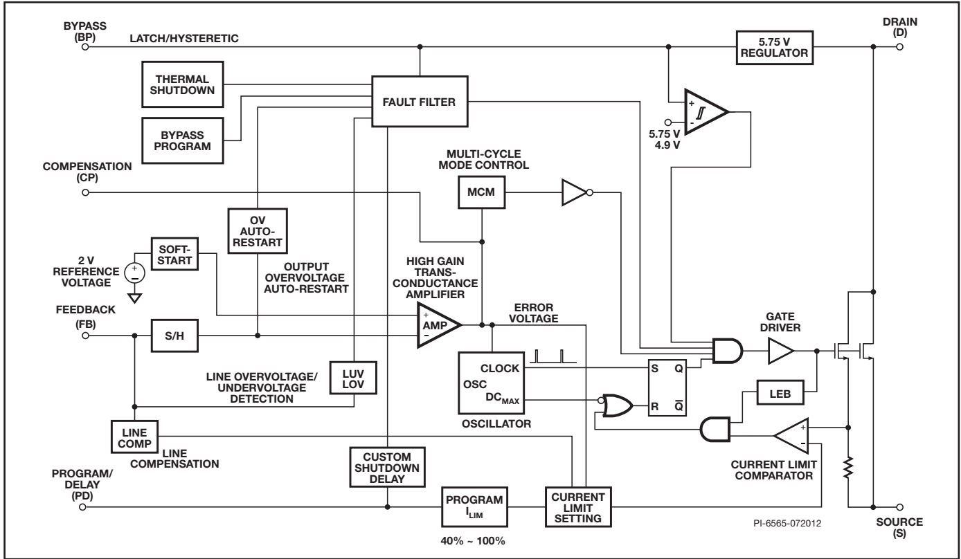
Figure 3. Block Diagram.
