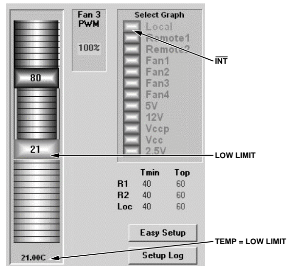
Figure 30. Temperature = Low Limit: \overline{\text{INT}} Occurs
