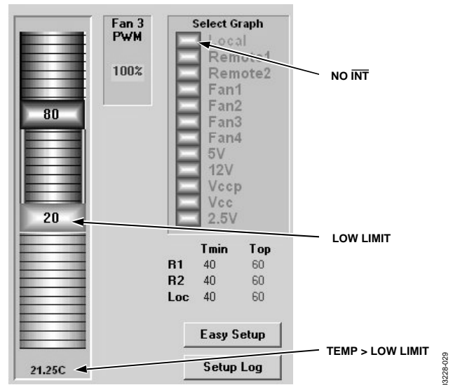
Figure 29. Temperature > Low Limit: No \overline{\text{INT}}
