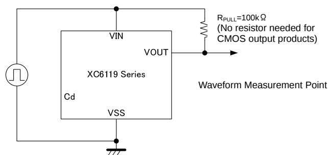
Circuit 8
