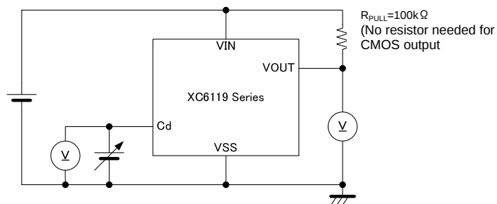
Circuit 8
