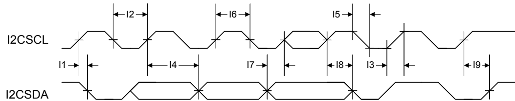
Figure 19-13. I 2 C Timing
