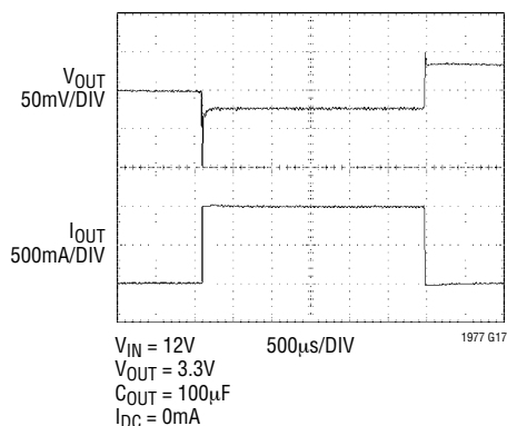
No Load 1A Step Response
