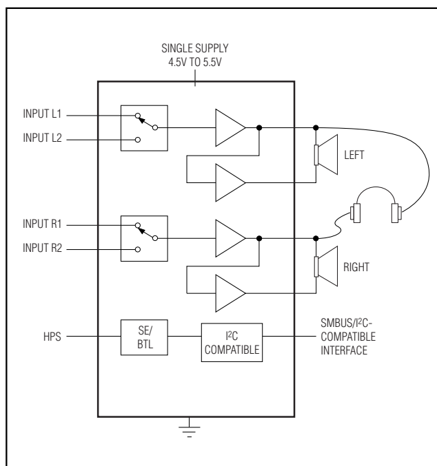
Figure 1. MAX9760/61 EV Kit Block Diagram
