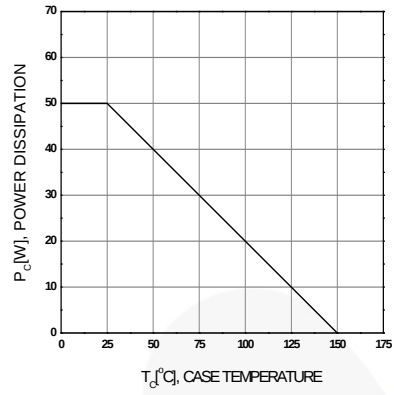
Figure 8. Power Derating
