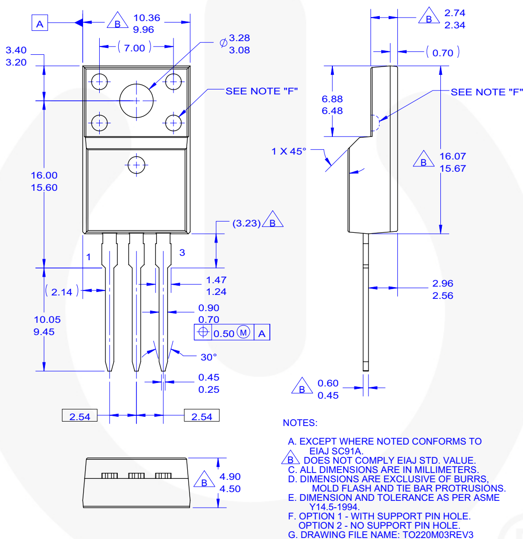
Figure 9. TO220, MOLDED, 3-LEAD, FULL PACK, EIAJ SC91, STRAIGHT LEAD (ACTIVE)
