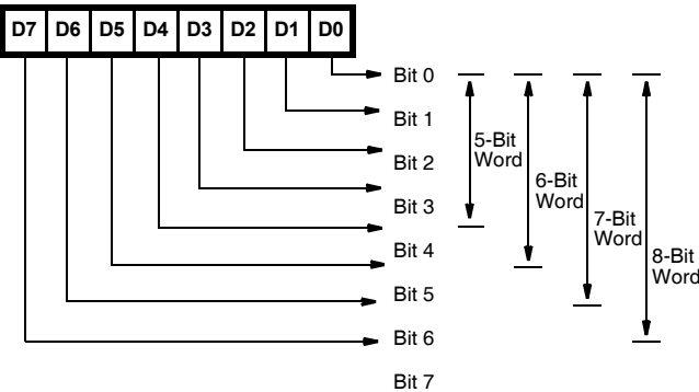
FIGURE 8. TBR
