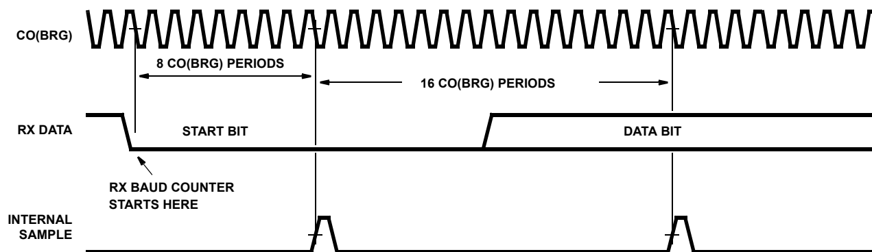
FIGURE 17. RECEIVER DATA
