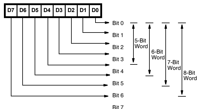
FIGURE 7. RBR
