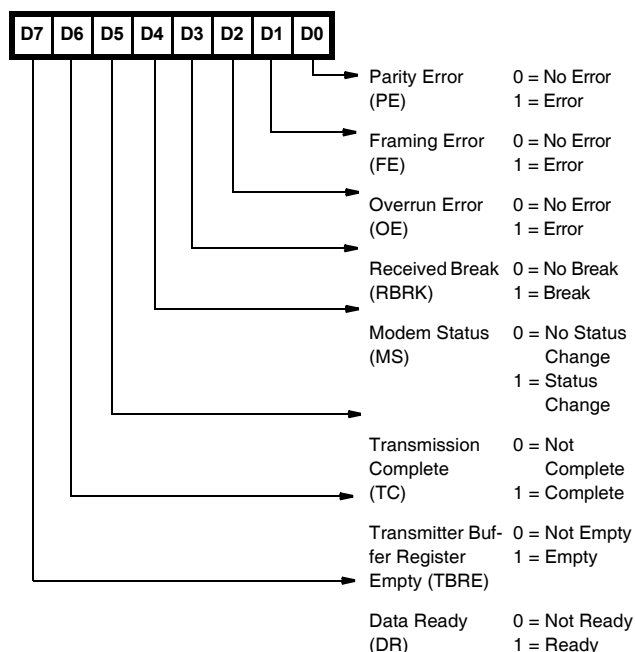
FIGURE 5. USR
