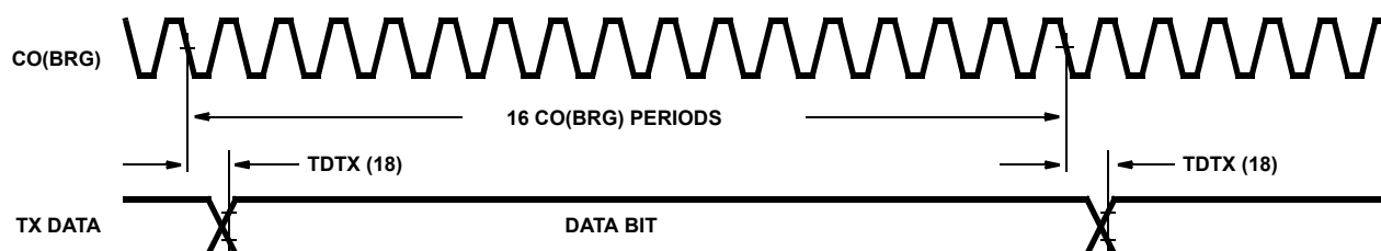
FIGURE 16. TRANSMITTER DATA
