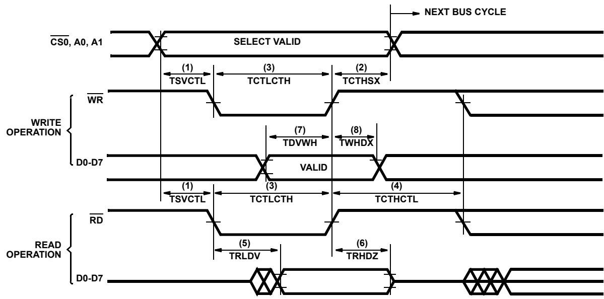
FIGURE 14. BUS OPERATION
