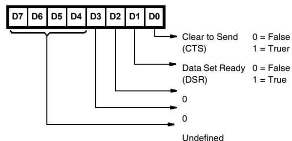
FIGURE 6. MSR
