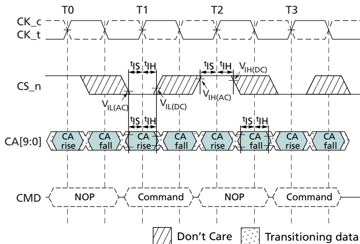
Figure 9: Command and Input Setup and Hold
