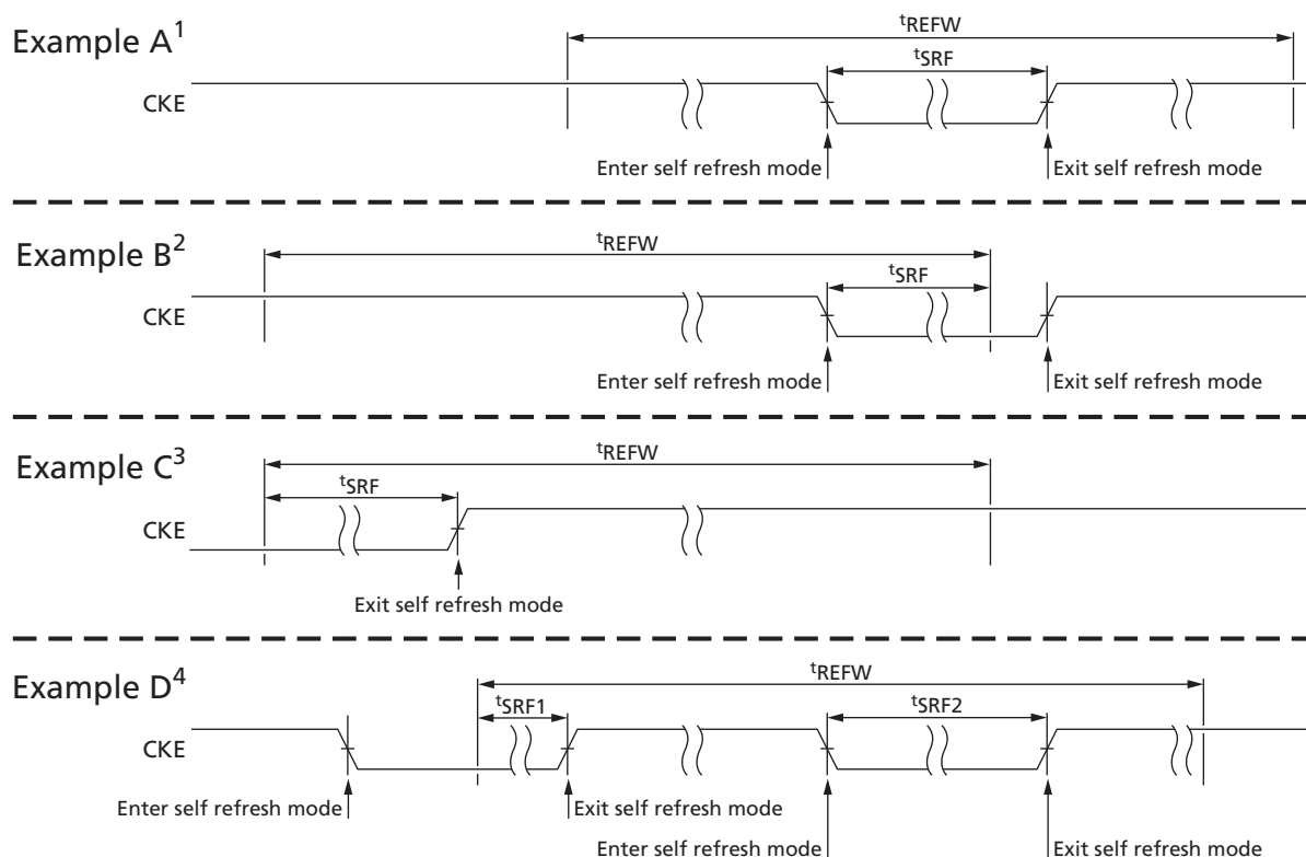
Figure 37: t_{SRF} Definition
