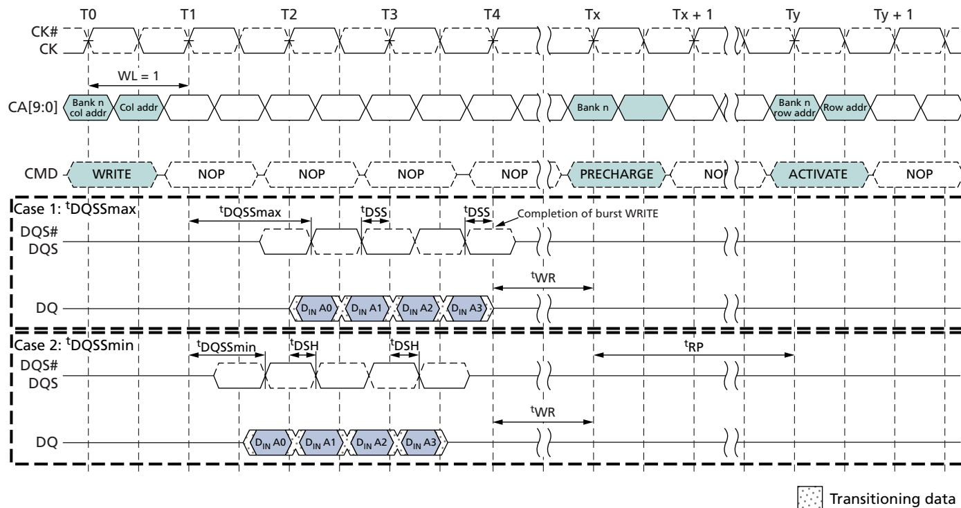
Figure 24: Burst WRITE – WL = 1, BL = 4
