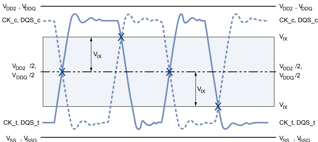
Figure 57: V_{IX} Definition
