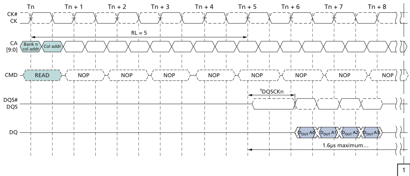
Figure 18: t_{DQSCDM} Timing
