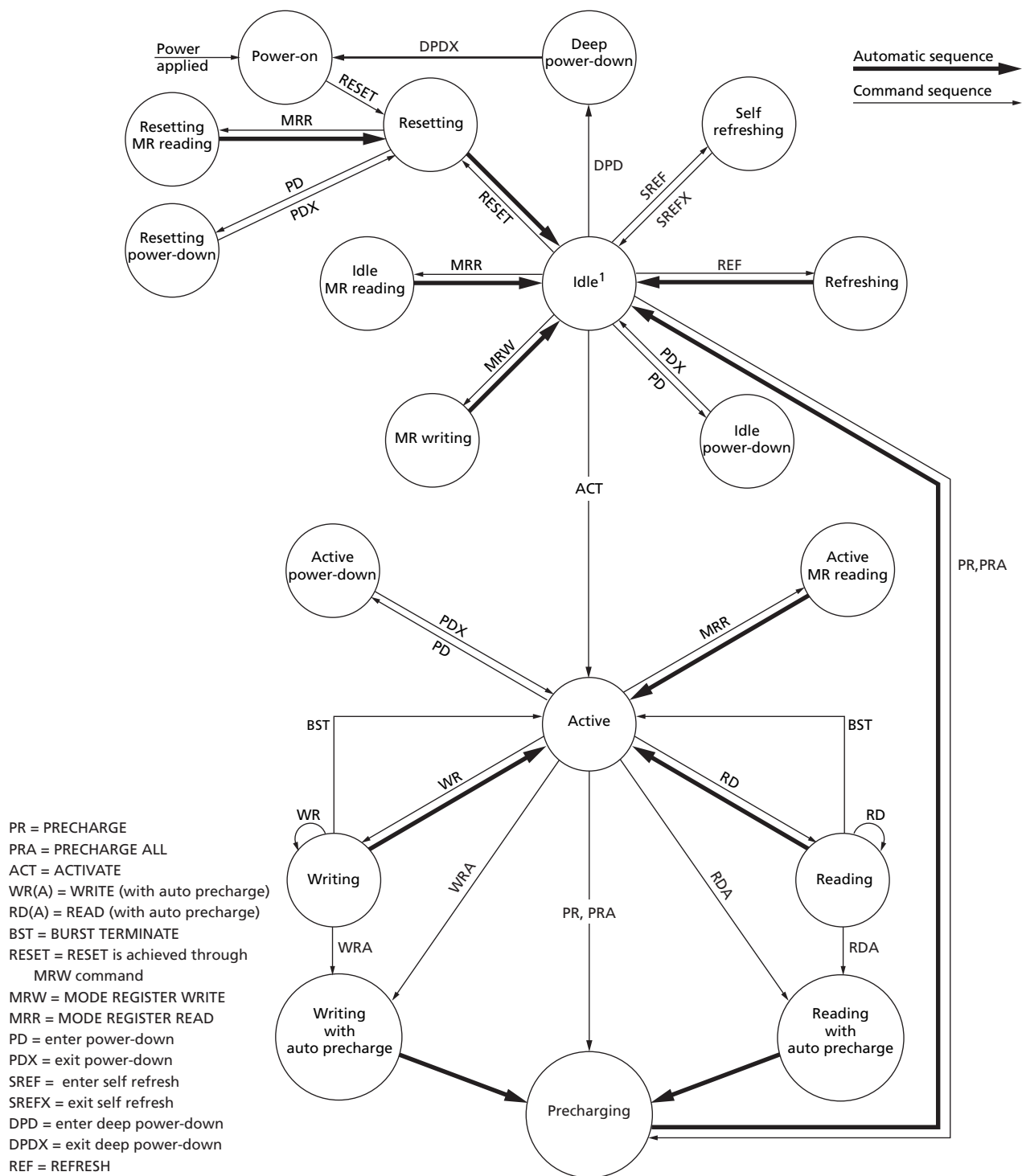
Figure 7: Simplified State Diagram
