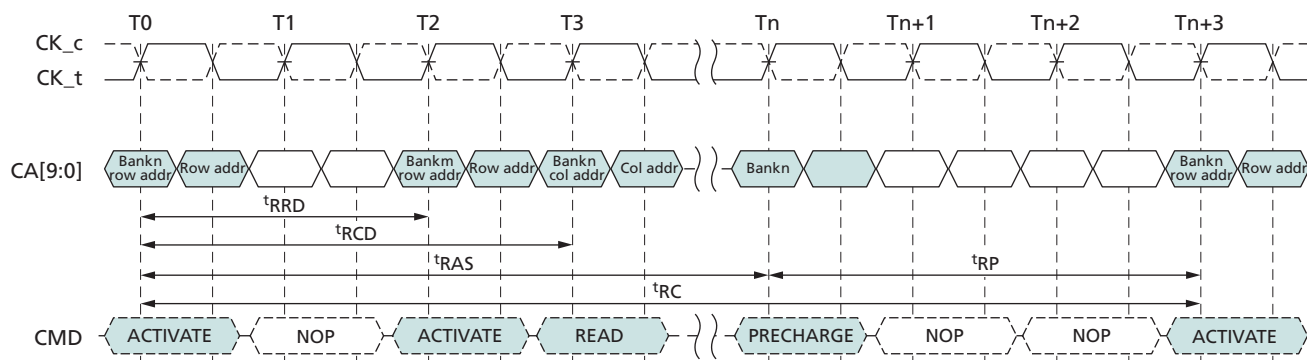
Figure 11: ACTIVATE Command
