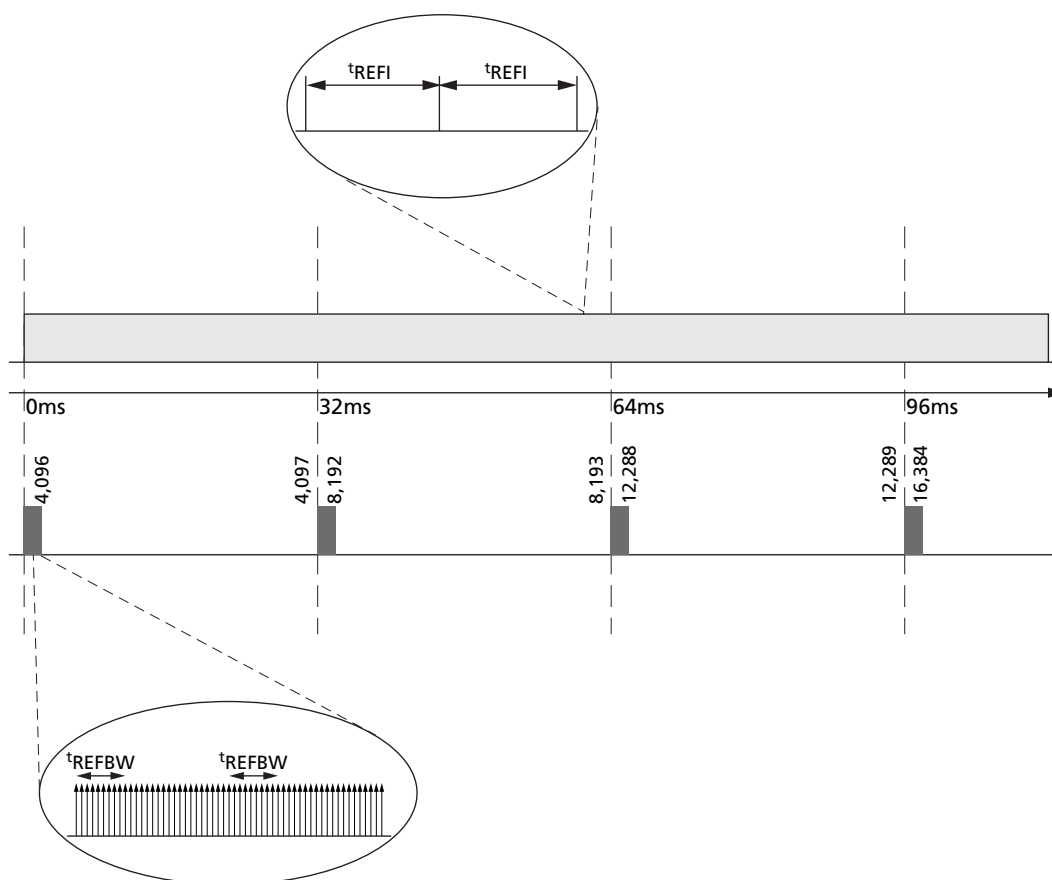
Figure 38: Regular Distributed Refresh Pattern
