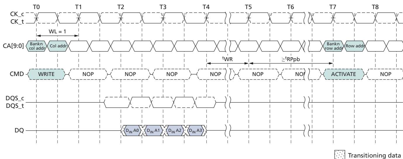
Figure 36: WRITE Burst with Auto Precharge – WL = 1, BL = 4
