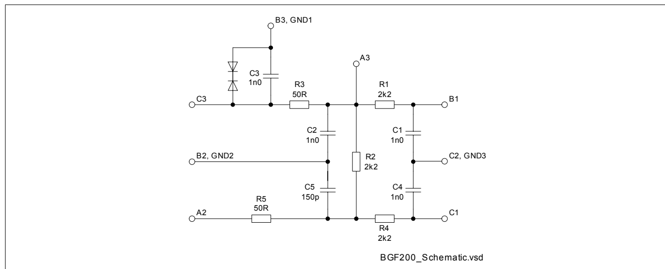
Figure 2 Schematic
