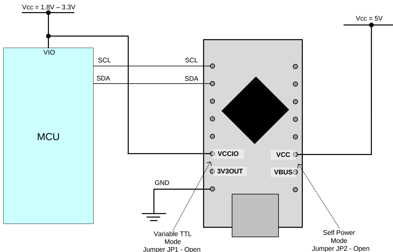
Figure 5.2 – Self-Powered Configuration
