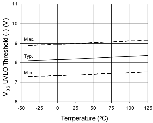
Figure 25. V_{BS} Undervoltage Threshold (-) vs. Temperature
