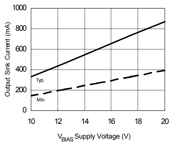
Figure 27B. Output Sink Currentt vs. Supply Voltage
