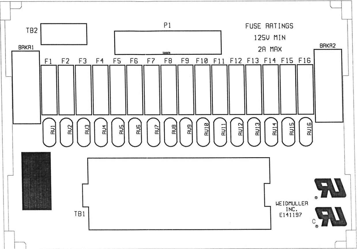
WTI-95020/67 REV. C SILKSCREEN ARTMASTER COMPONENT SIDE
