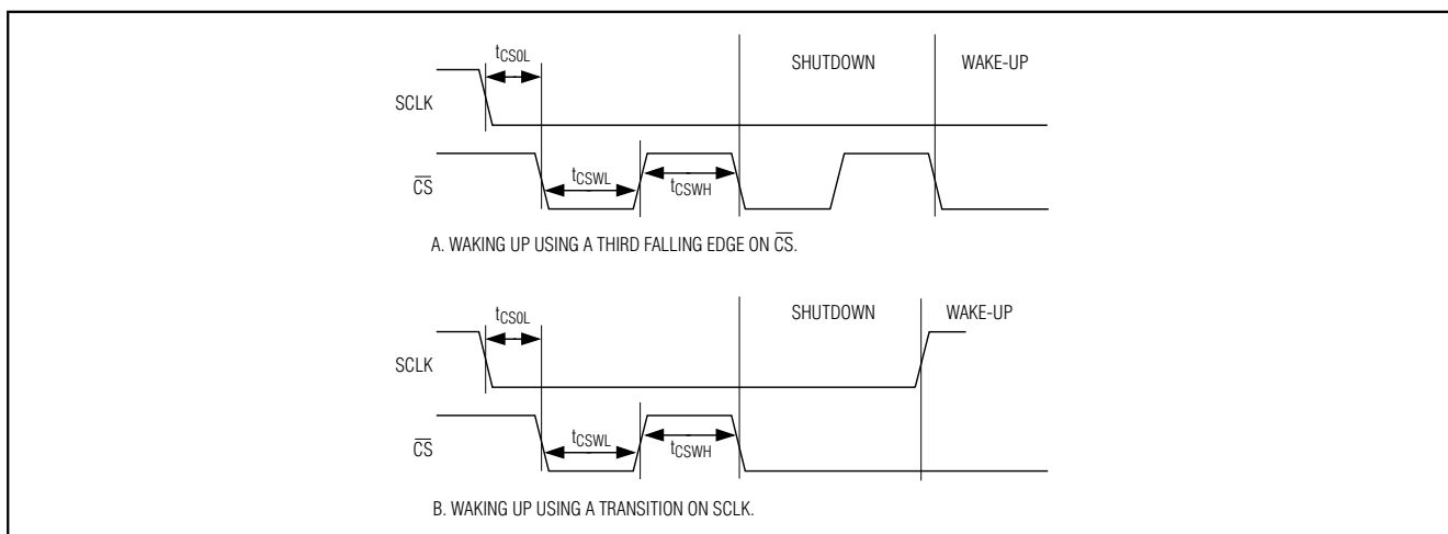
Figure 4. Shutdown Timing
