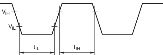
Figure 20.3 Input Timing
