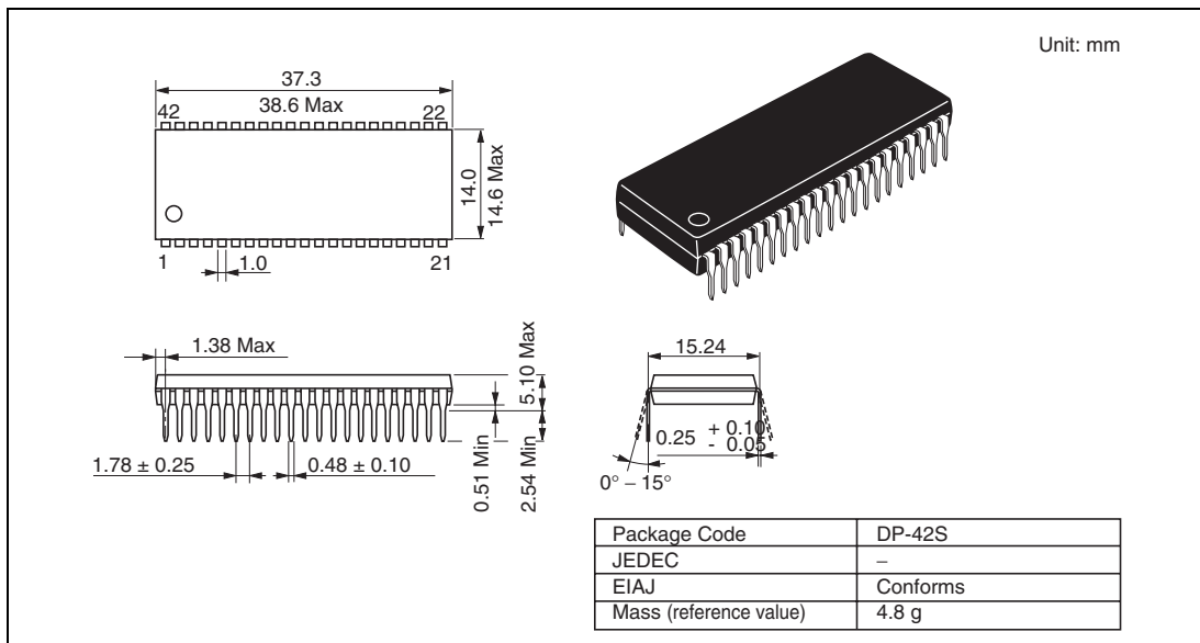
Figure D.5 DP-42S Package Dimensions
