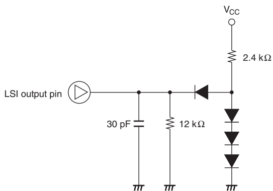
Figure 20.8 Output Load Circuit
