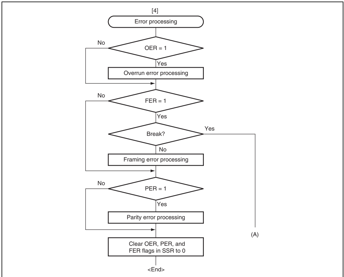
Figure 14.8 Sample Serial Reception Data Flowchart (2)
