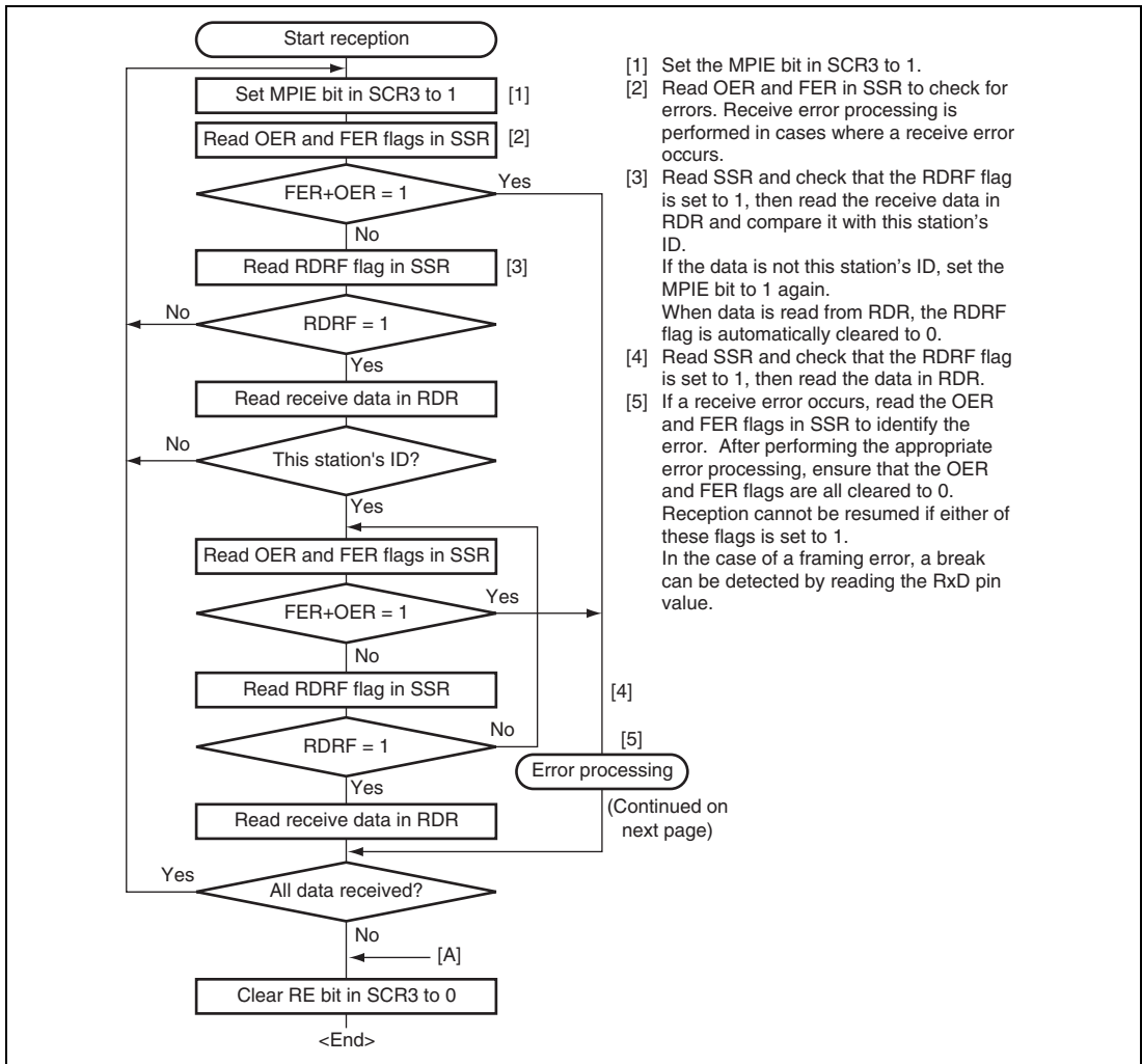
Figure 14.17 Sample Multiprocessor Serial Reception Flowchart (1)
