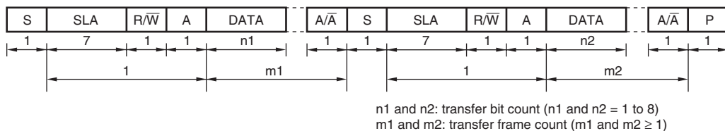
Figure 15.3 I 2 C Bus Data Formats (I 2 C Bus Formats)
