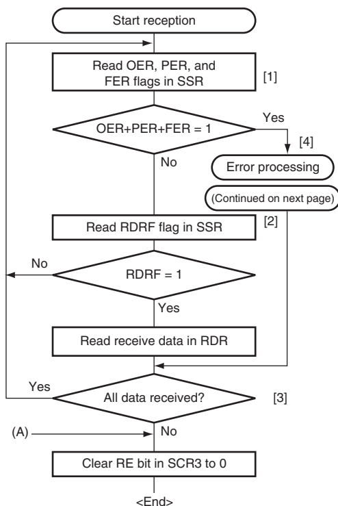
Figure 14.8 Sample Serial Data Reception Flowchart (Asynchronous mode) (1)
