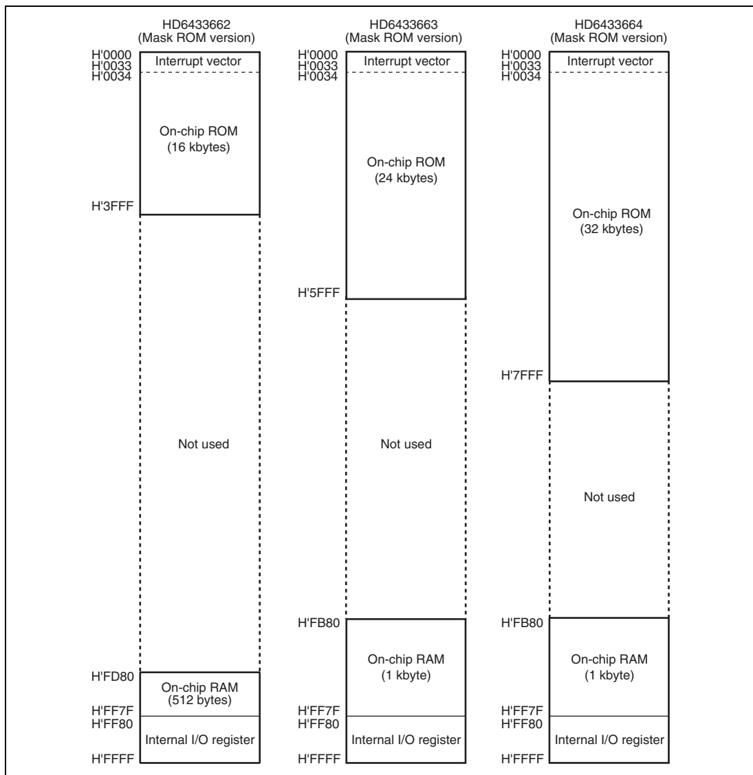
Figure 2.1 Memory Map (2)
