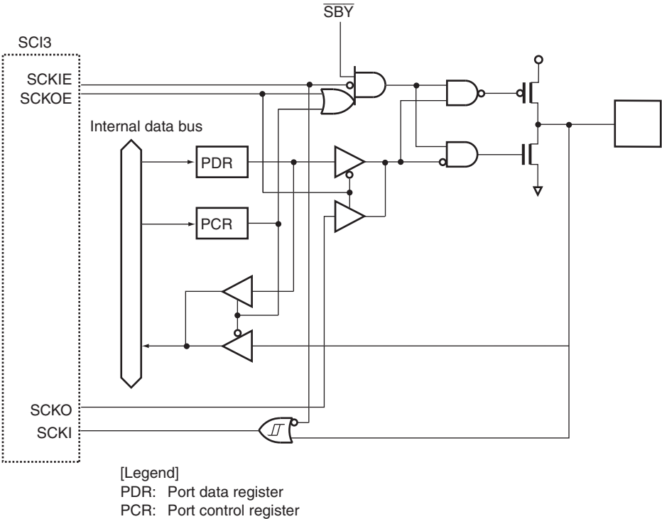
Figure B.7 Port 2 Block Diagram (P20)
