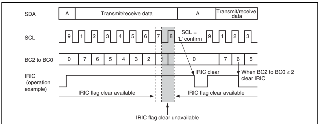
Figure 15.18 IRIC Flag Clear Timing on WAIT Operation
