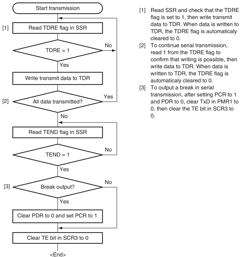
Figure 14.6 Sample Serial Transmission Flowchart (Asynchronous Mode)
