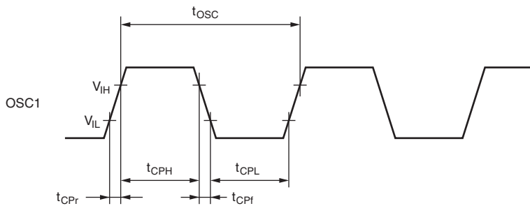
Figure 20.1 System Clock Input Timing
