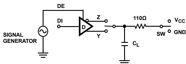
FIGURE 5. DRIVER PROPAGATION DELAY AND DIFFERENTIAL TRANSITION TIMES
