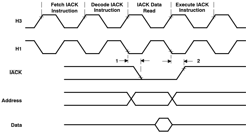
Figure 22. \overline{\text{IACK}} Timing
