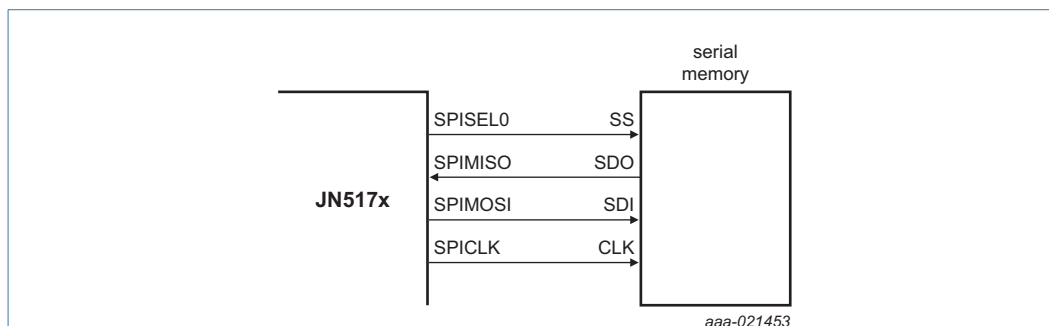
Fig 8. Connecting external serial memory
