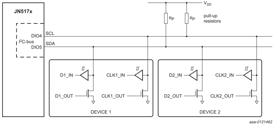
Fig 34. Connection details
