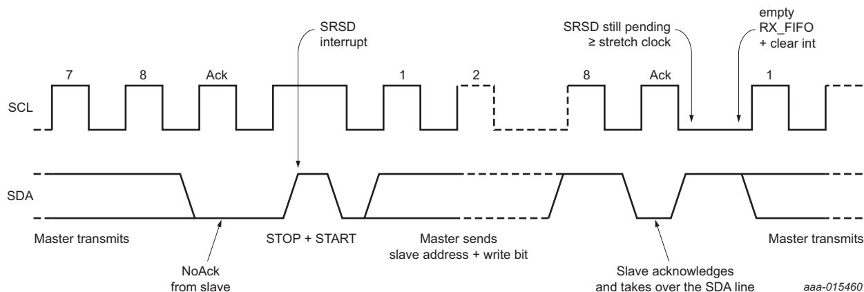
Fig 40. Example of use of the SRSD interrupt (STOP case)
