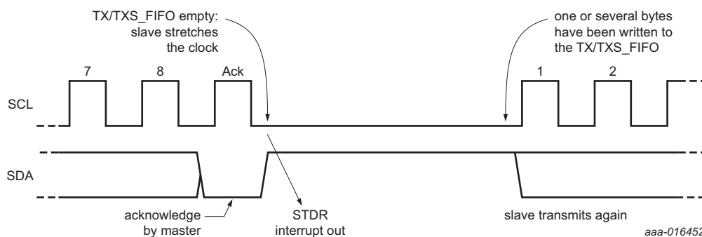
Fig 41. TXS FIFO empty in the middle of a transaction
