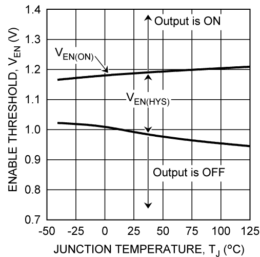
Figure 4. Enable Thresholds
