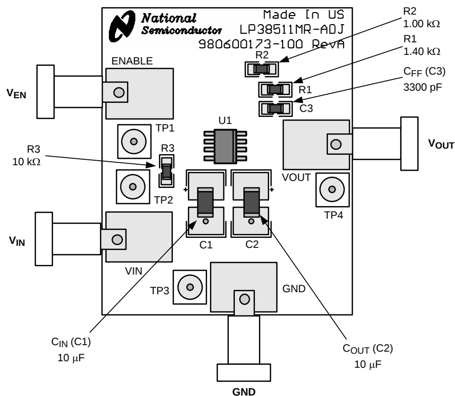
Figure 8. Evaluation Board Component and Pin Layout
