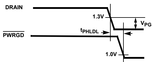
FIGURE 4A. DRAIN TO PWRGD ACTIVE TIMING (ISL6142)
