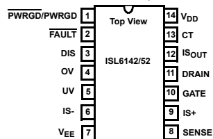
ISL6142 OR ISL6152 (14 LEAD SOIC)
