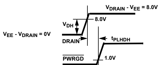
FIGURE 6A. DRAIN HIGH TO PWRGD (INACTIVE) HIGH (ISL6142)
