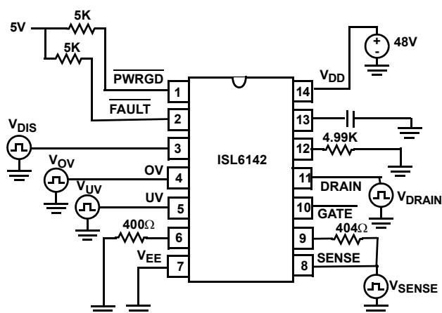
FIGURE 2A. TYPICAL TEST CIRCUIT
