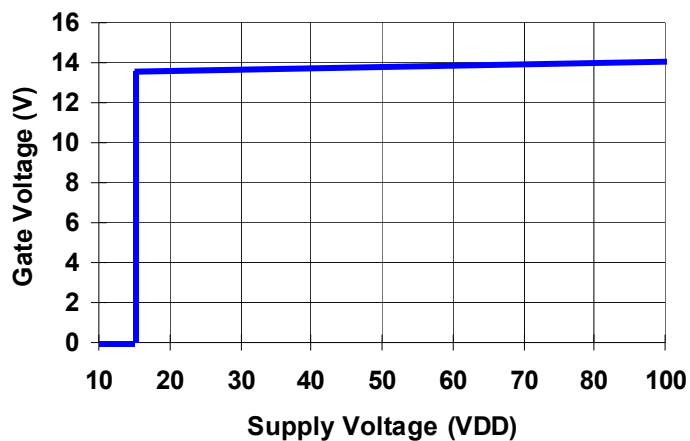
FIGURE 14. GATE VOLTAGE VS SUPPLY VOLTAGE (25°C)
