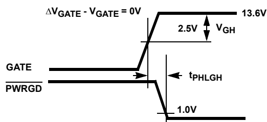
FIGURE 5A. GATE TO PWRGD ACTIVE (ISL6142)
