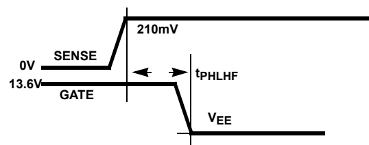
FIGURE 10. SENSE TO GATE (HARD FAULT) TIMING
