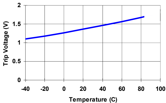
FIGURE 23. DRAIN to PWRGD / PWRGD TRIP VOLTAGE ( V_{PG} ) VS TEMPERATURE
