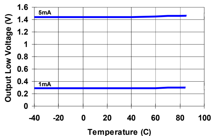
FIGURE 22. PWRGD (ISL6142) VOL VS TEMPERATURE
