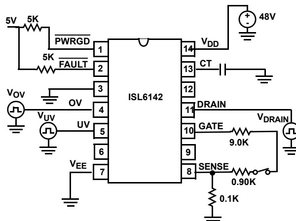
FIGURE 2B. TEST CIRCUIT FOR TIMEOUT
