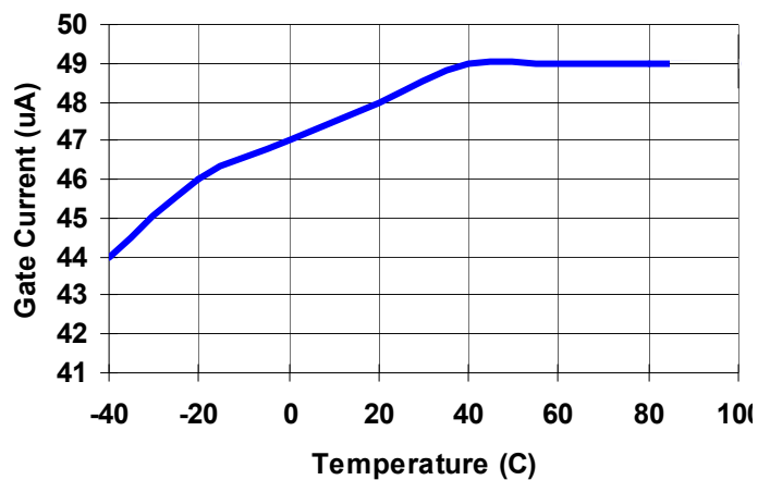
FIGURE 18. GATE PULL-UP CURRENT VS TEMPERATURE
