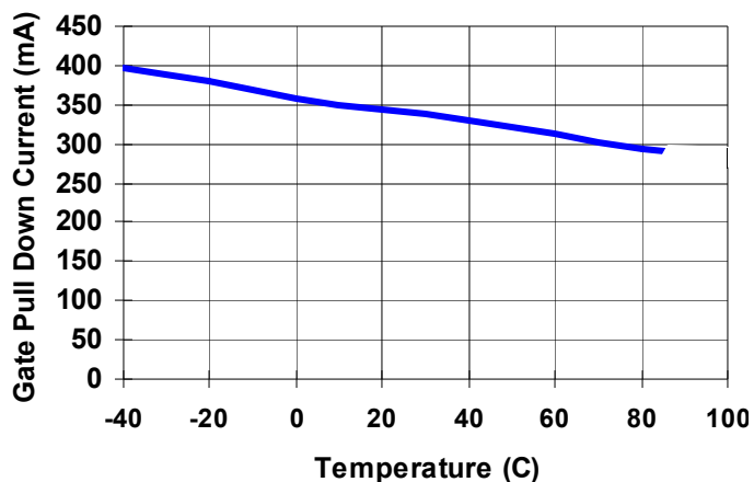
FIGURE 20. HARD FAULT GATE PULL-DOWN CURRENT VS TEMPERATURE
