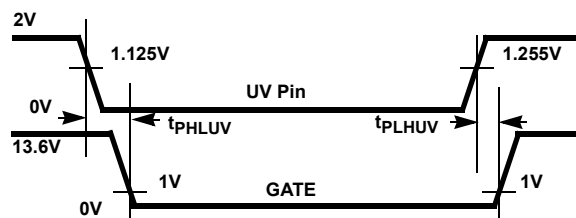
FIGURE 3B. UV TO GATE TIMING
