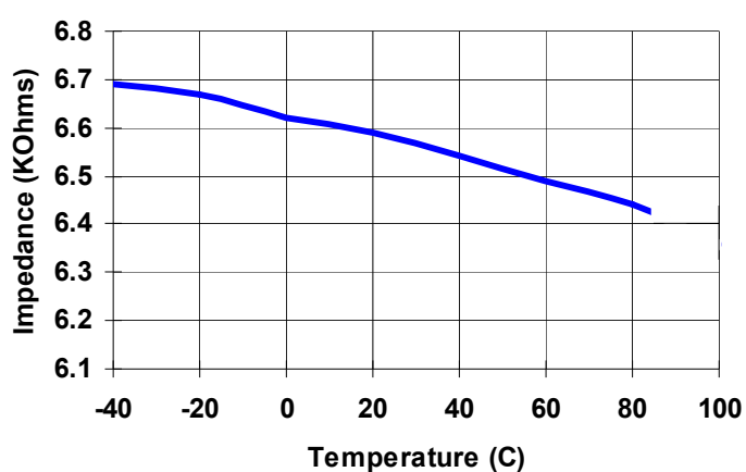
FIGURE 24. PWRGD (ISL6152) OUTPUT IMPEDANCE VS TEMPERATURE
