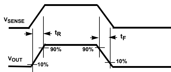
FIGURE 10. SENSE TO GATE (HARD FAULT) TIMING
