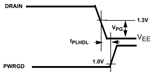
FIGURE 4B. DRAIN TO PWRGD ACTIVE TIMING (ISL6152)
