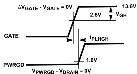
FIGURE 5B. GATE TO PWRGD ACTIVE (ISL6152)
