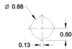
30.5mm Detail (1490 Series) 22.5mm Detail (1490M Series)
