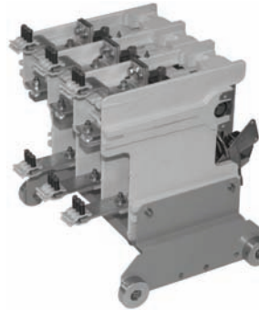
Stab-In AMPGARD 800A Contactor—Rear View
