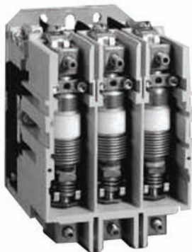
Size 4 Vacuum Contactors
