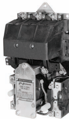
Type N Contactor
