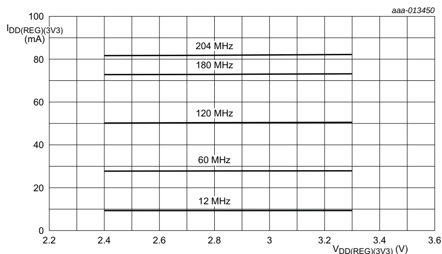
Fig 11. Typical supply current versus regulator supply voltage V_{DD(REEG)(3V3)} in active mode
