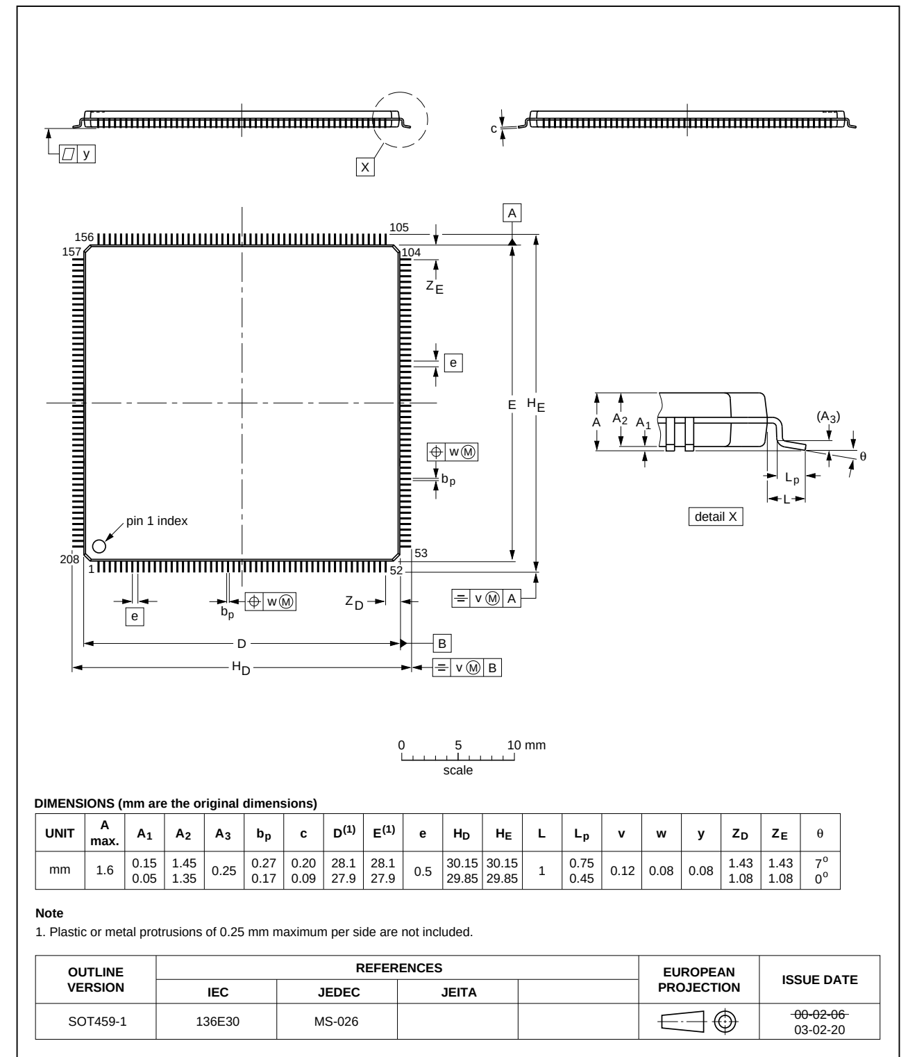
Fig 52. Package outline of the LQFP208 package
