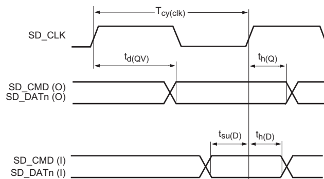
Fig 40. SD/MMC timing
