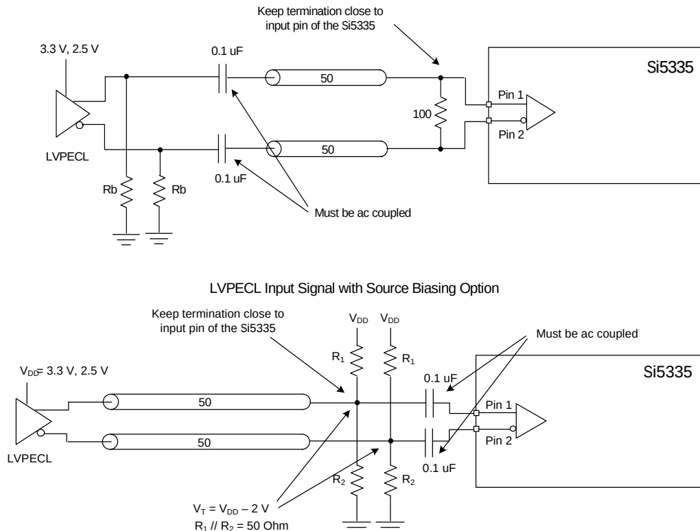
Figure 6. Recommended Options for Interfacing to an LVPECL Input Signal
