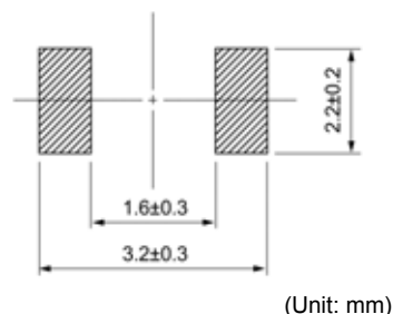
Recommended patterns 推荐焊盘尺寸
