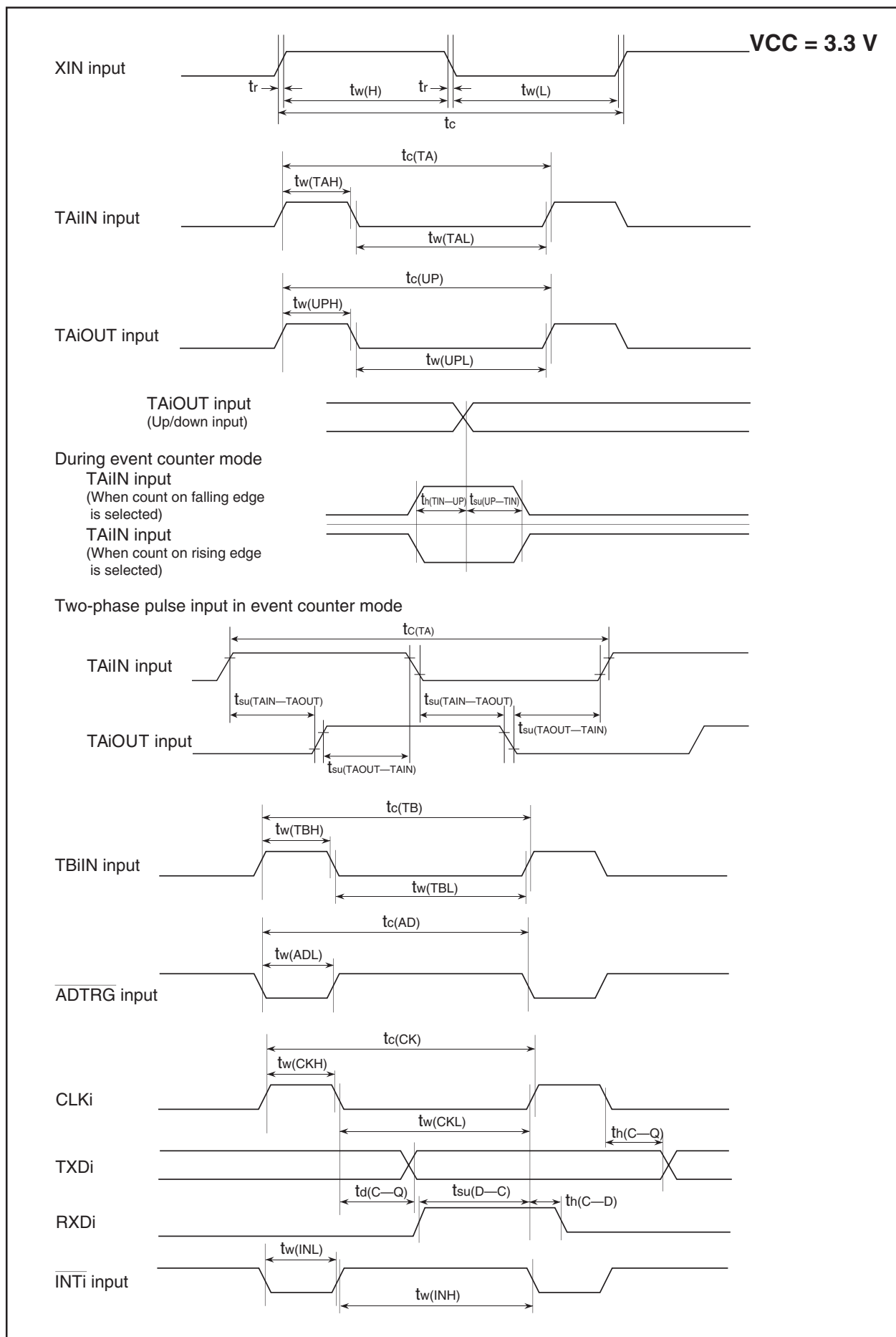
Figure 5.12 Timing Diagram (1)
