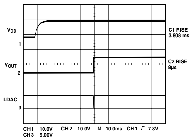
Figure 8. Turn-On Characteristics
