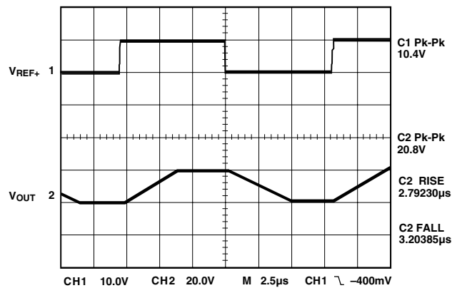
Figure 4. Pulse Response (Large Signal)
