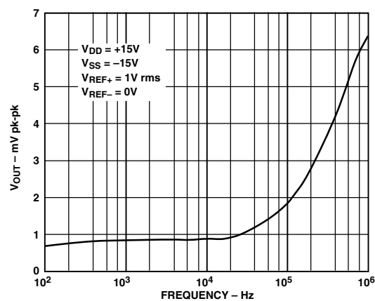
Figure 1b. AC Feedthrough vs. Frequency
