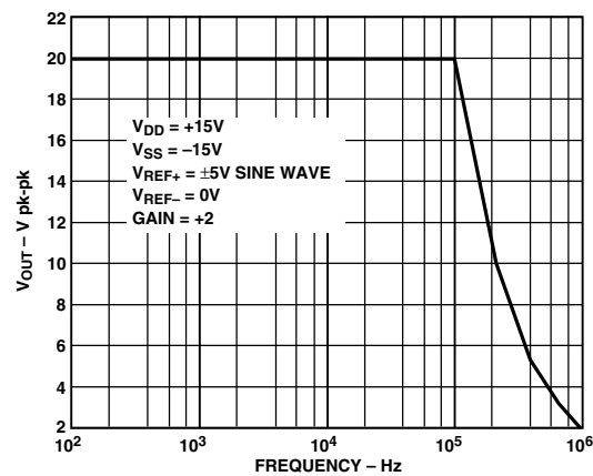
Figure 3. Large Signal Frequency Response
