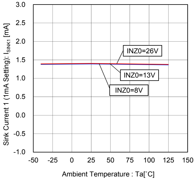
Figure 37. Sink Current 1 (1mA Setting) vs Ambient Temperature
