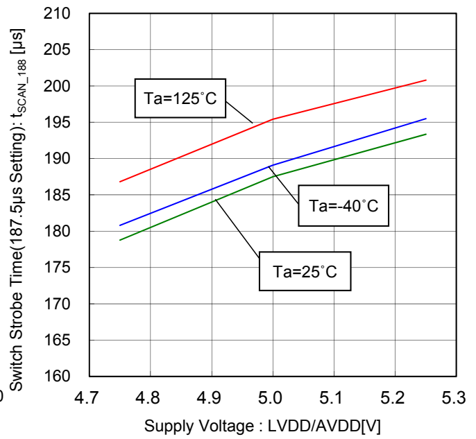
Figure 114. Switch Strobe Time(187.5μs Setting) vs Supply Voltage
