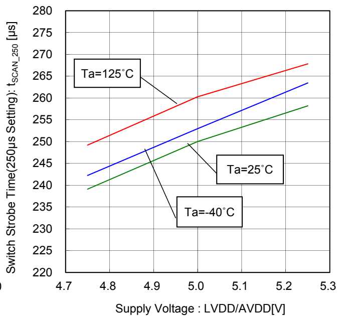
Figure 116. Switch Strobe Time(250μs Setting) vs Supply Voltage
