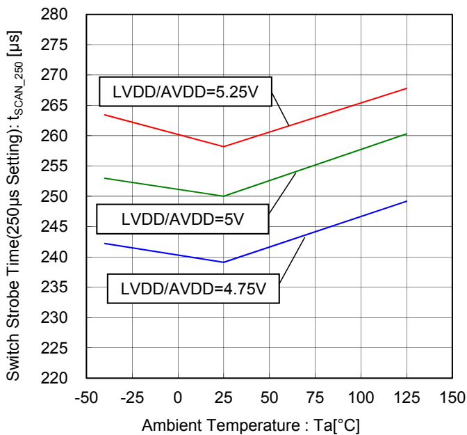
Figure 115. Switch Strobe Time(250μs Setting) vs Ambient Temperature
