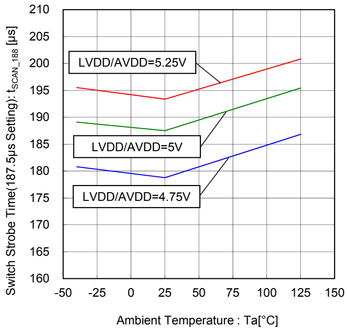
Figure 113. Switch Strobe Time(187.5μs Setting) vs Ambient Temperature
