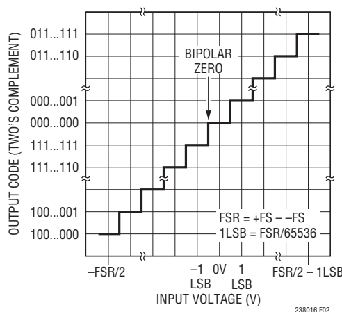
Figure 2. LTC2380-16 Transfer Function
