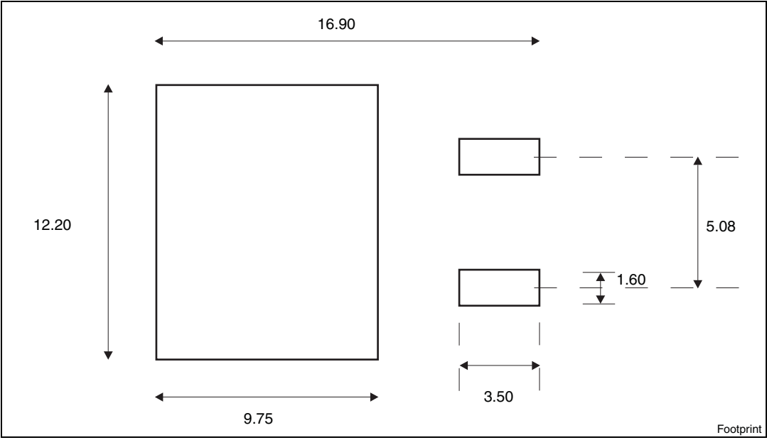
Figure 28. D²PAK footprint (a)
