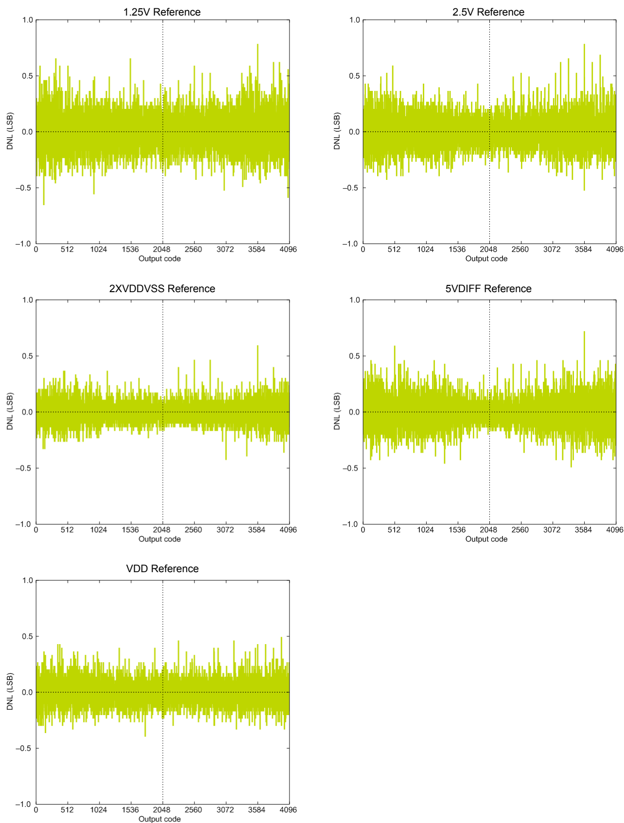
Figure 4.30. ADC Differential Linearity Error vs Code, VDD = 3 V, Temp = 25 °C
