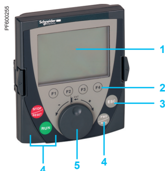
Remote graphic display terminal
