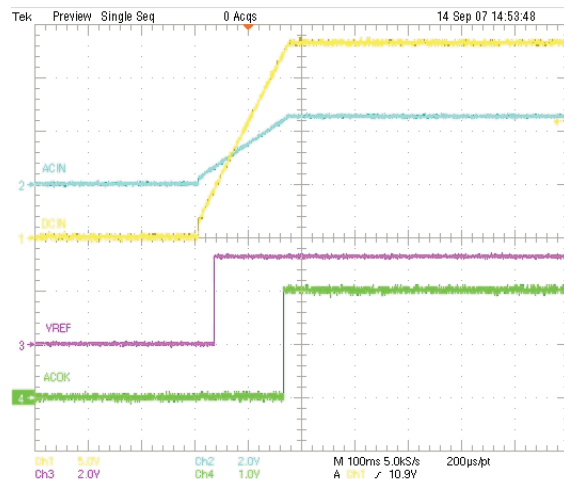
Figure 20. Charger When Adapter Inserted
