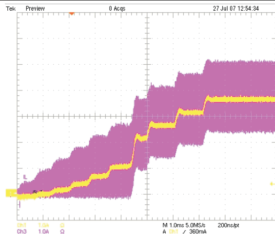
Figure 22. Inductor Current and Battery Current Soft-Start
