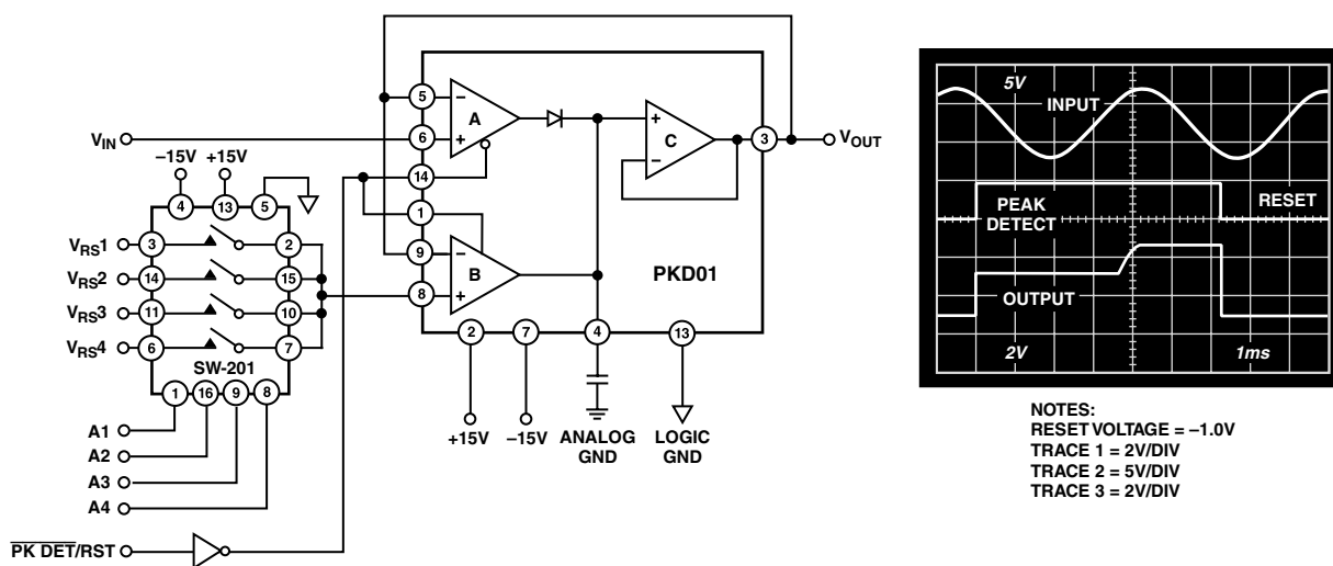
Figure 21. Positive Peak Detector with Selectable Reset Voltage
