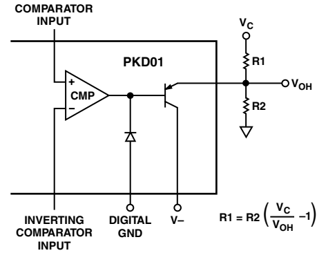
Figure 10. Comparator Output with External Level-Setting Resistors
