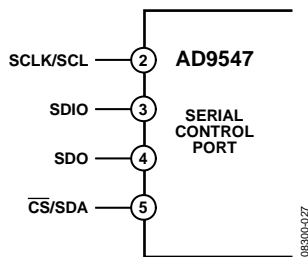
Figure 50. Serial Control Port
