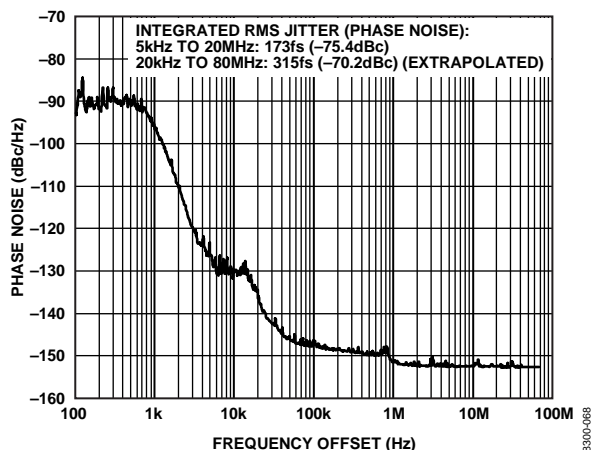
Figure 3. Additive Phase Noise (Output Driver = LVPECL), f_{REF} = 19.44 MHz, f_0 = 155.52 MHz, LBW = 1 kHz, f_{SYSCLK} = 1 GHz, PLL Off
