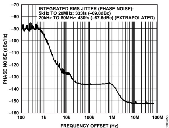
Figure 4. Additive Phase Noise (Output Driver = LVPECL), f_{REF} = 19.44 MHz, f_0 = 155.52 MHz, LBW = 1 kHz, f_{SYSCLK} = 50 MHz (Crystal), PLL On
