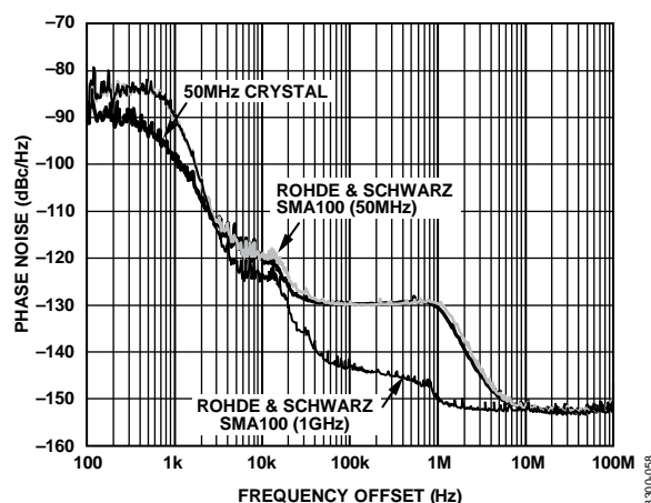
Figure 10. Additive Phase Noise Comparison of SYSCLK Input Options (Output Driver = LVPECL), f_{REF} = 19.44 MHz, f_0 = 311.04 MHz, LBW = 1 kHz
