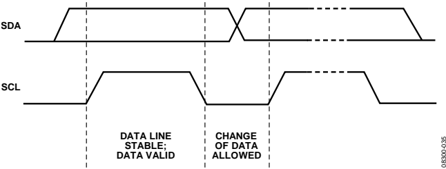
Figure 57. Valid Bit Transfer
