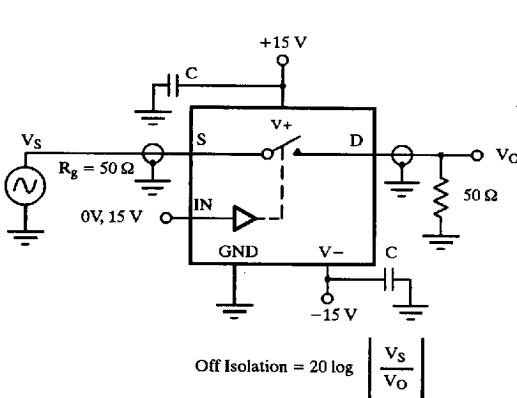
Figure 3. Off Isolation
