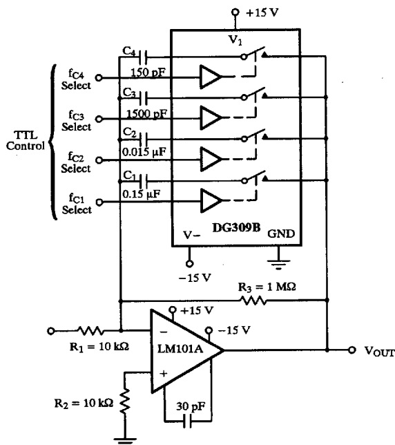
Figure 9. Active Low Pass Filter with Digitally Selected Break Frequency
