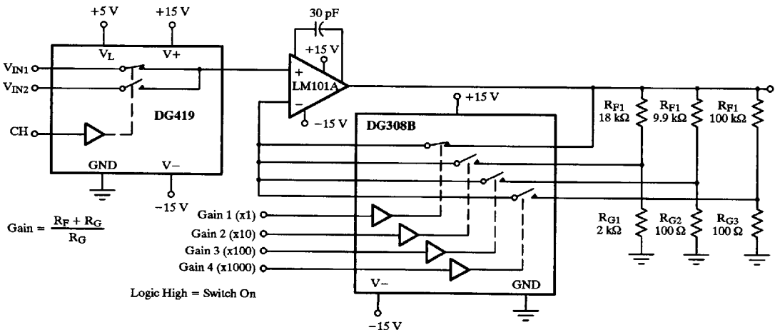
Figure 7. A Precision Amplifier with Digitally Programmable Inputs and Gains
