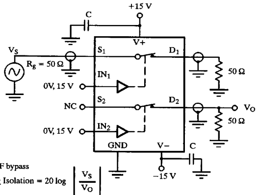
Figure 4. Channel-to-Channel Crosstalk
