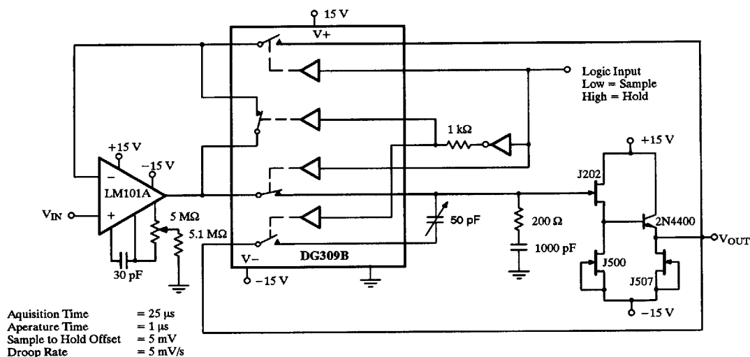
Figure 8. Sample-and-Hold
