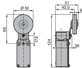
Rubber Roller Lever
