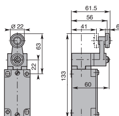
Roller Lever Nylon
