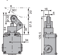
Adjustable Rubber Roller Lever
