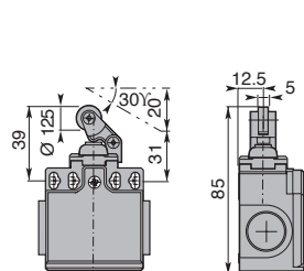
Plastic Roller
