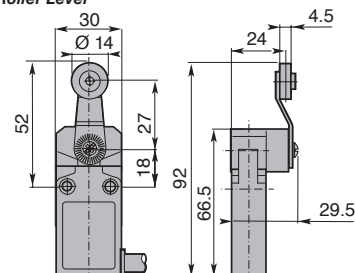
Roller Lever
