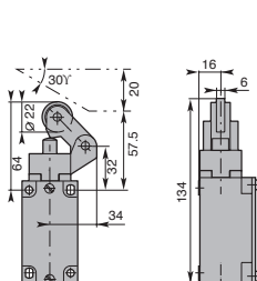
One way Roller
