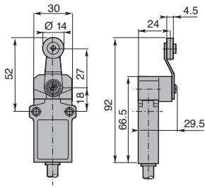
Roller Lever
