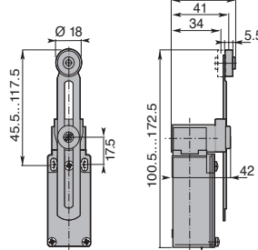
Adjustable Roller Lever
