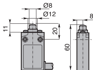
Plain Plunger
