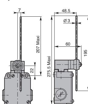
Adjustable Rod Lever
