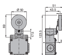
Adjustable Lever with Adjustable Rubber Roller
