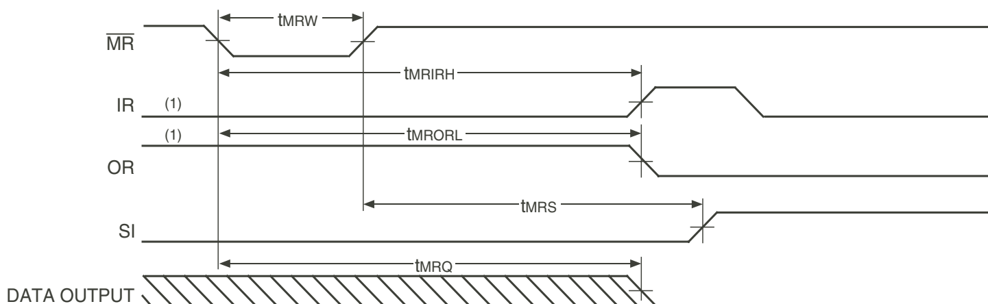
Figure 8. Master Reset Timing
