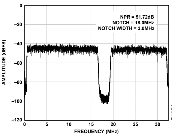
Figure 41. Noise Power Ratio (NPR), f_{\text{SAMPLE}} = 65 \text{ MSPS}
