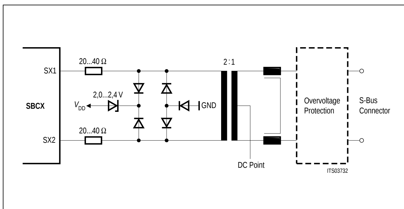
Figure 80 External Circuitry Transmitter
