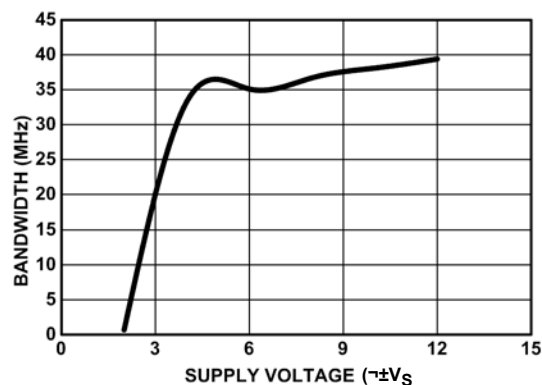
FIGURE 11. DIFFERENTIAL 3dB BANDWIDTH vs SUPPLY VOLTAGE
