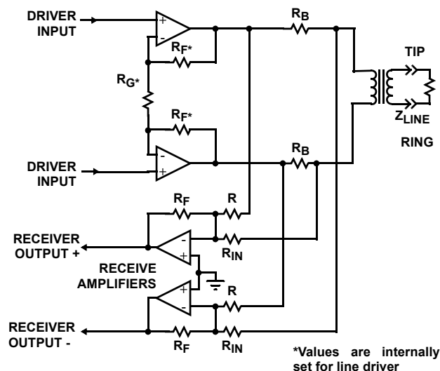
FIGURE 15. TYPICAL INTERFACE CIRCUIT CONFIGURATION
