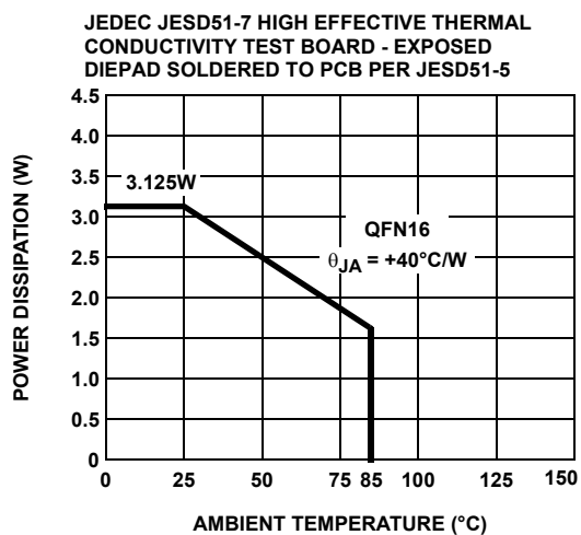
FIGURE 14. PACKAGE POWER DISSIPATION vs AMBIENT TEMPERATURE
