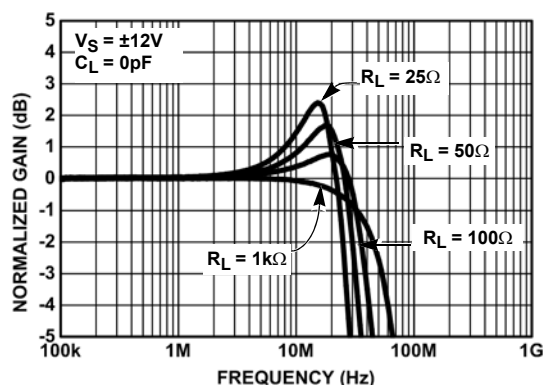
FIGURE 1. DIFFERENTIAL FREQUENCY RESPONSE vs R_L
