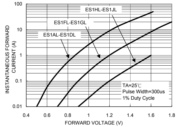
FIG. 2 TYPICAL FORWARD CHARACTERISRICS
